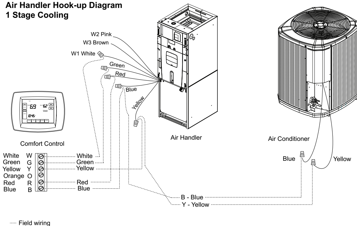
Air Handler Hook-up Diagram 1 Stage HP
