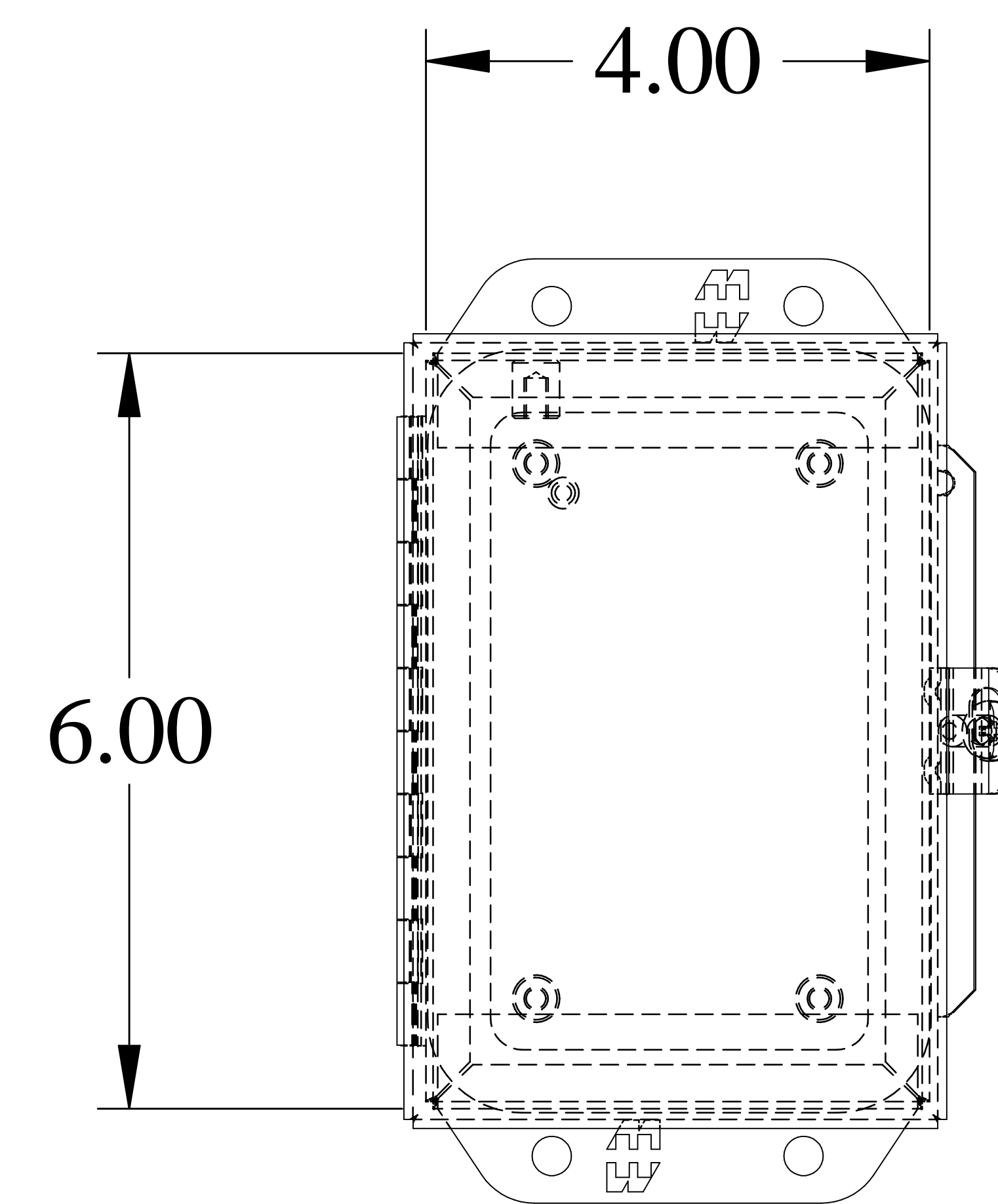
FRONT VIEW
