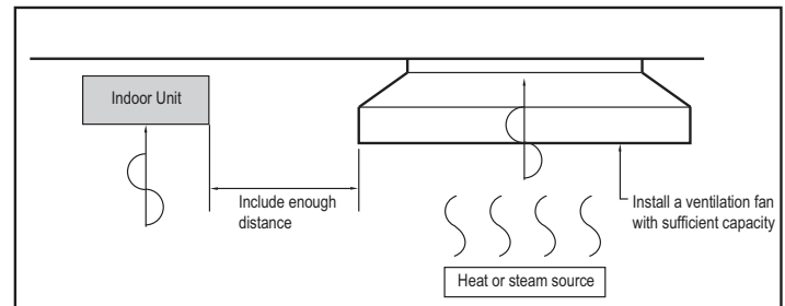
Figure 26: Installing Near a Heat or Steam Source.
