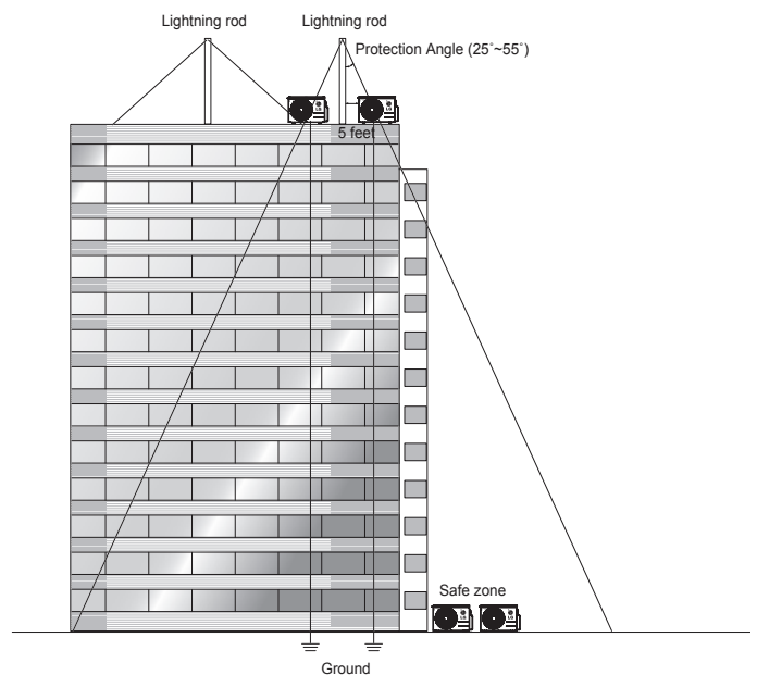
Figure 28: Lightning Protection Diagram.
