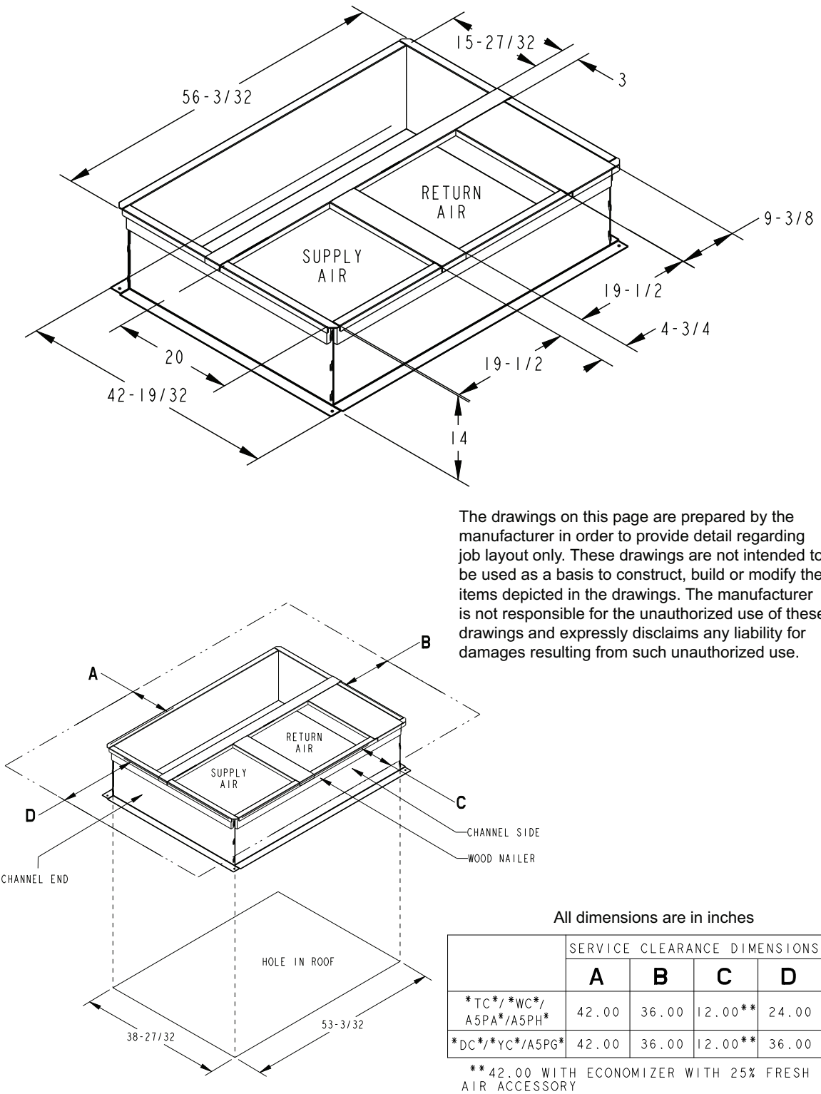
BAYCURB051B Full Perimeter Roof Mounting Curb
